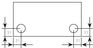
Typical Conduit Hole Location. Size = 25mm Conduit Knockouts
